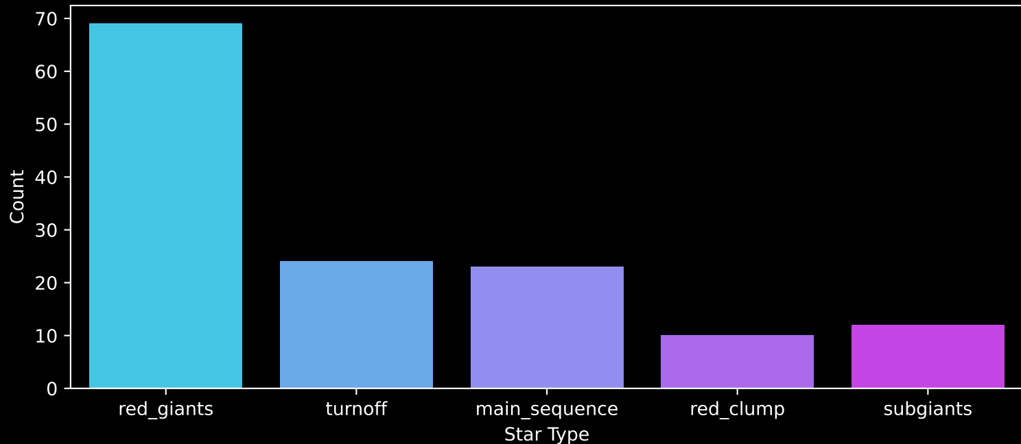
APOGEE DR17 Field: [TAUL1495] Count plot of Star Type
