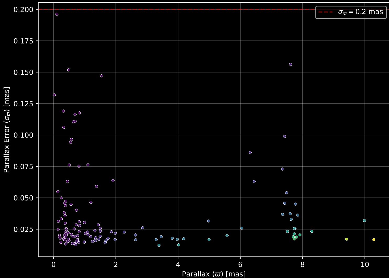
APOGEE DR17 Field: [TAUL1495] Parallax Quality (n= 138)
