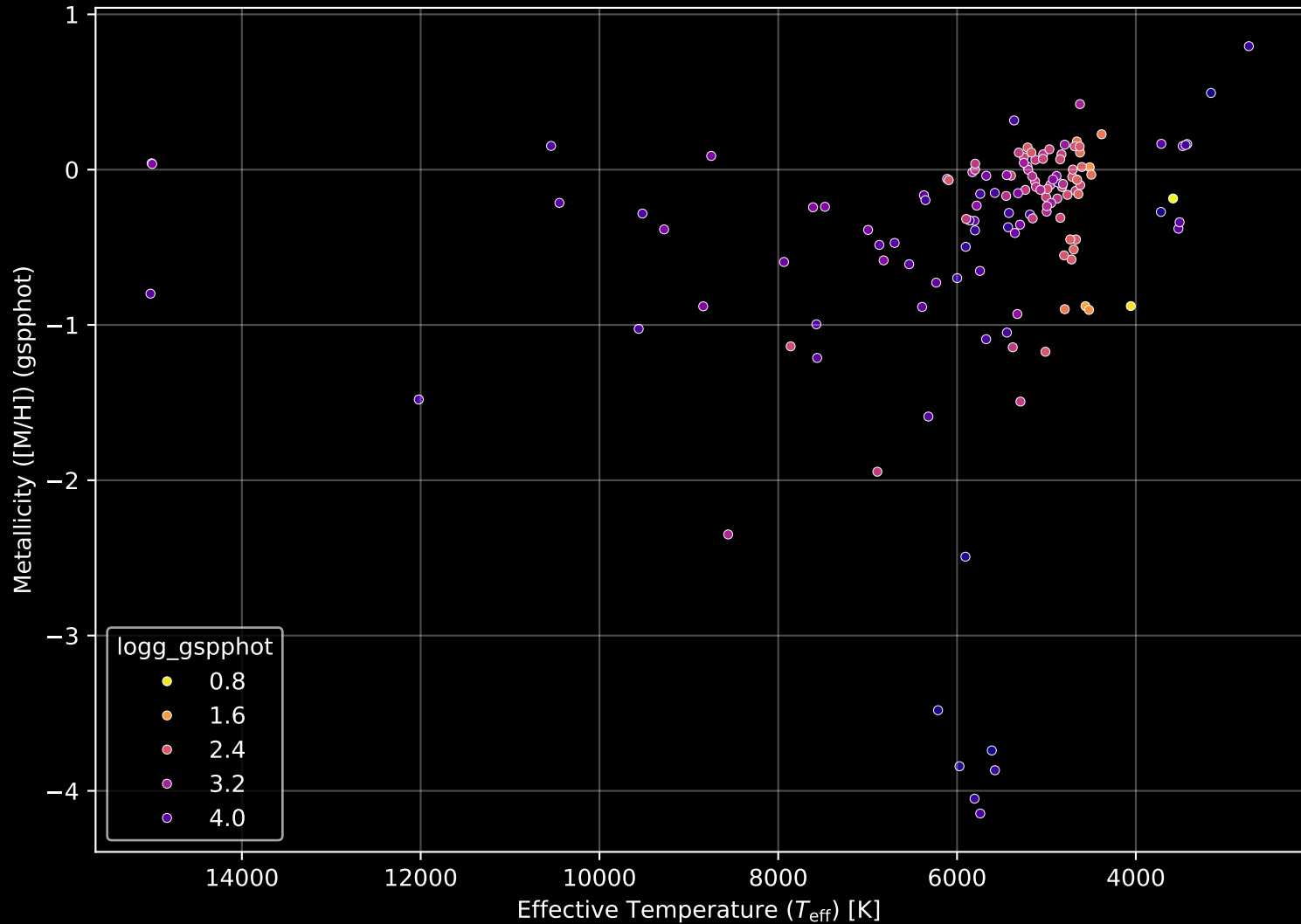
APOGEE DR17 Field: [TAUL1495] Stellar Population Parameters (n= 138)
