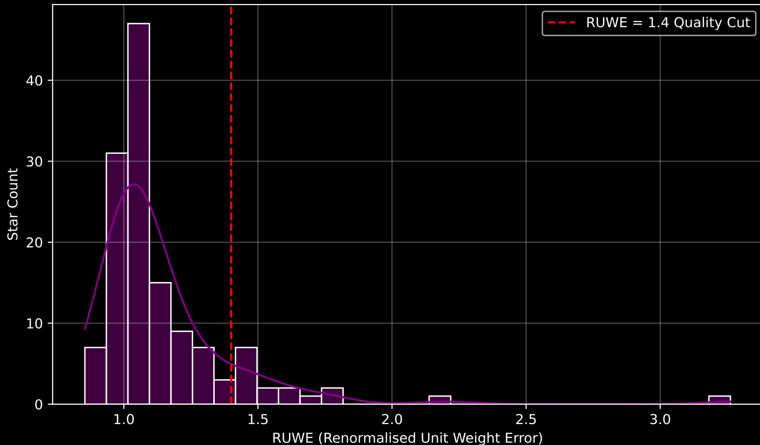
GAPOGEE DR17 Field [TAUL1495] RUWE Distribution (n= 135)
