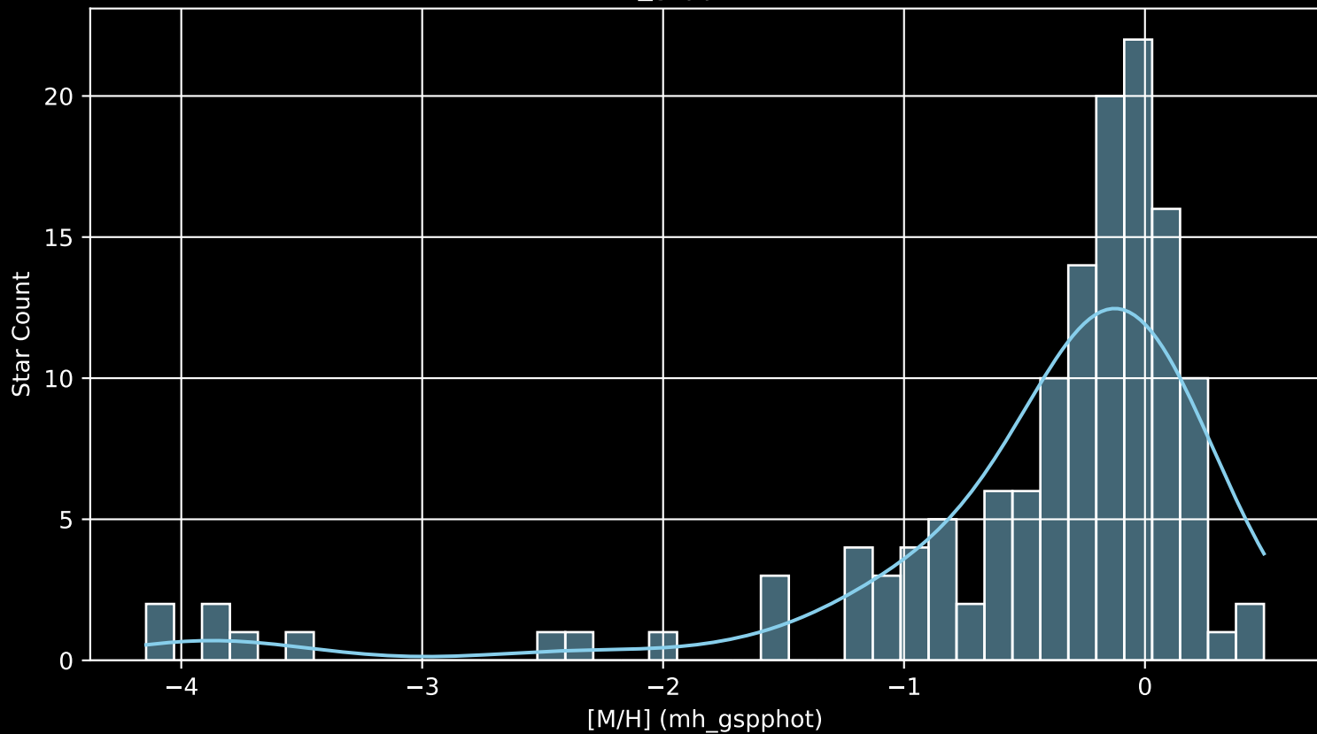
APOGEE DR17 Field: [TAUL1495 [M/H] (mh_gspphot) (n= 137)
