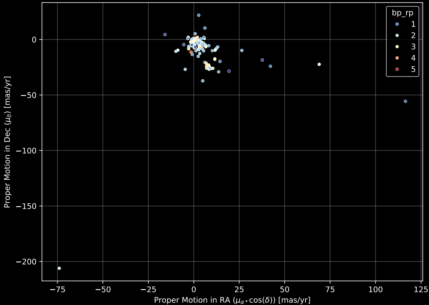
APOGEE DR17 Field: [TAUL1495] Proper Motion Diagram (n= 138)
